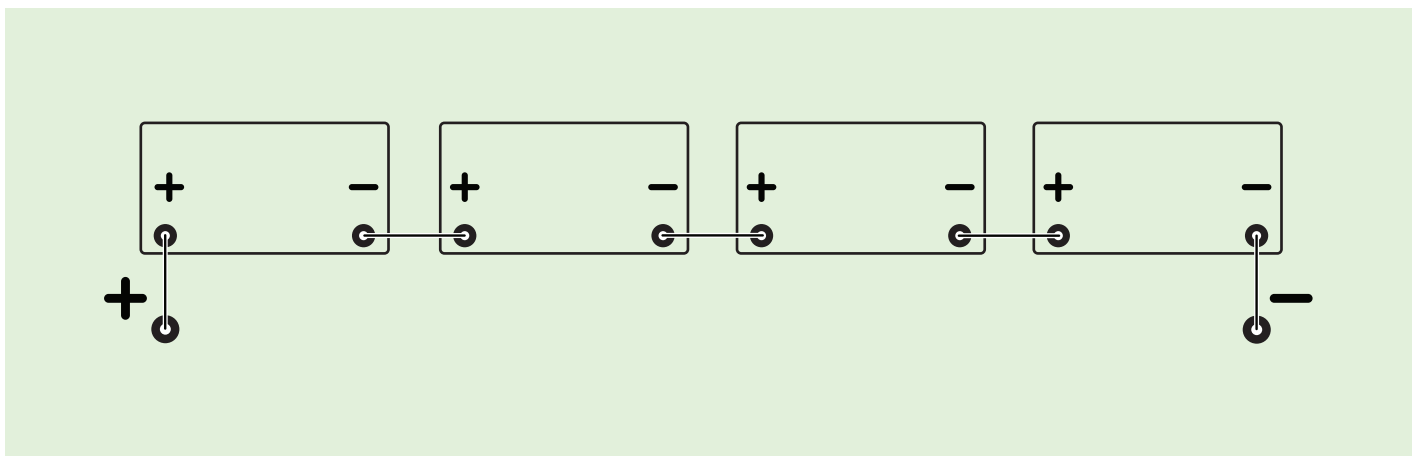
Figure 2: Connecting LFP Batteries in Series
